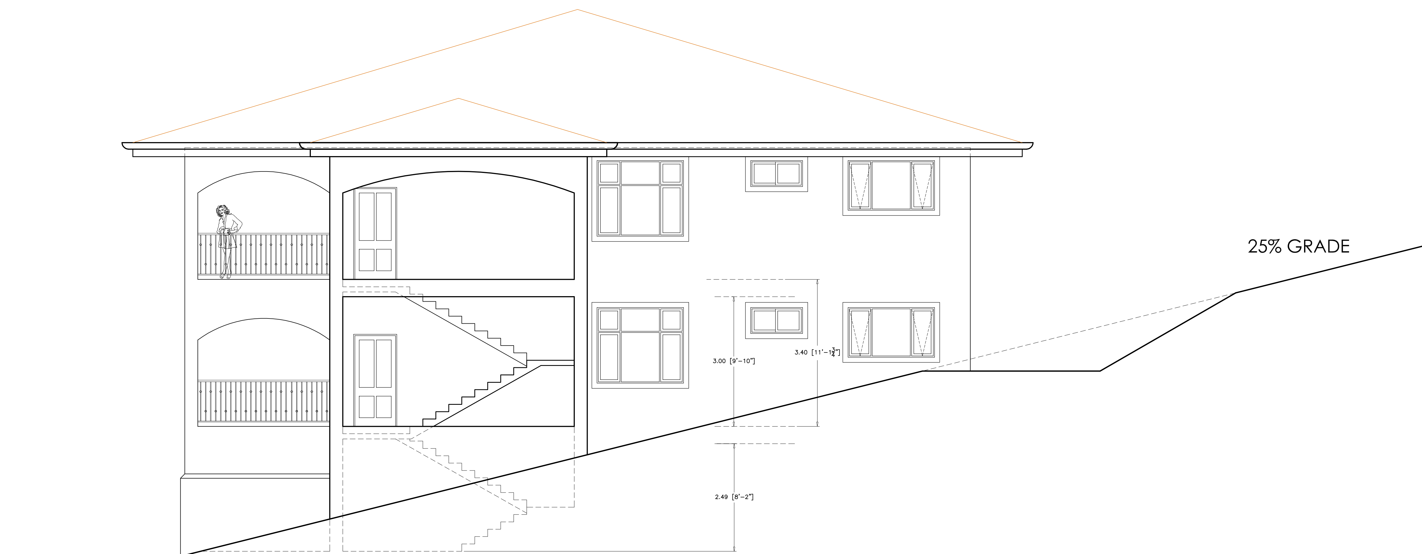
SIDE ELEVATION SCALE 1:50
